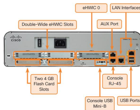
Back Panel of a Router
